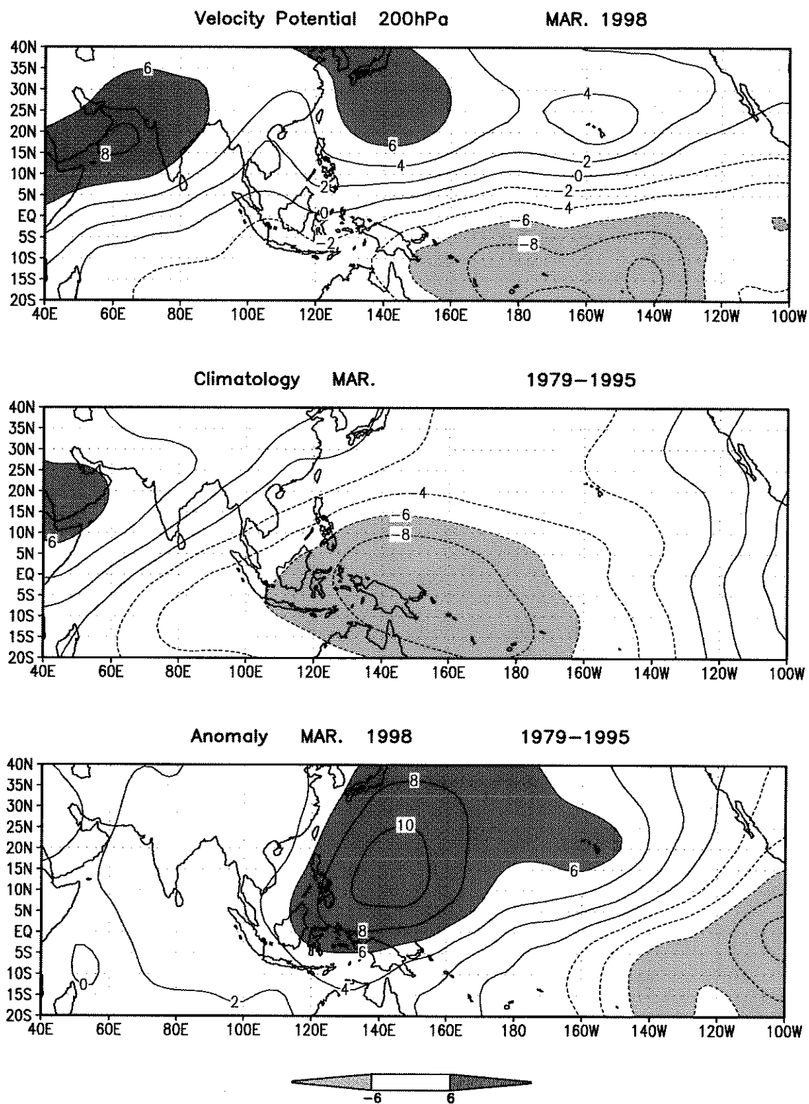
Figure 7b Same as Fig. 7a but for in March 1998.
