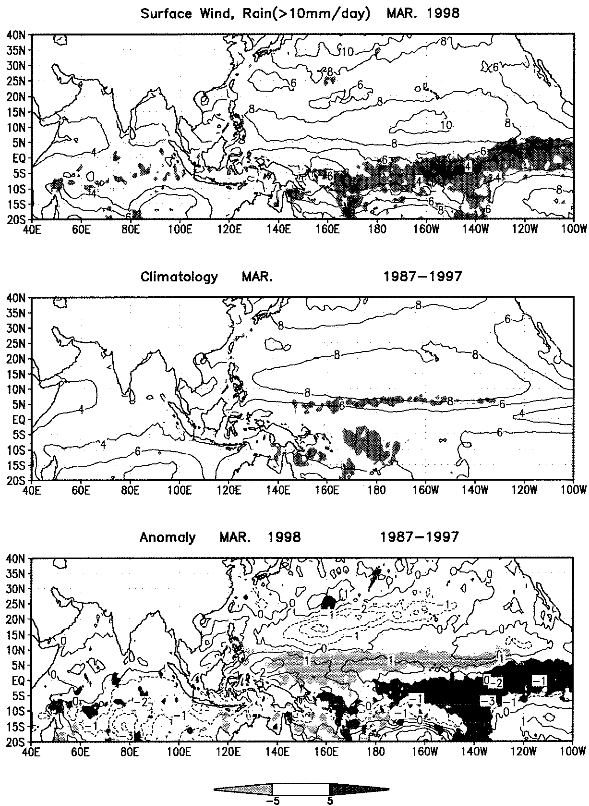
Figure 3b Same as Fig. 3a but for in March 1998.
