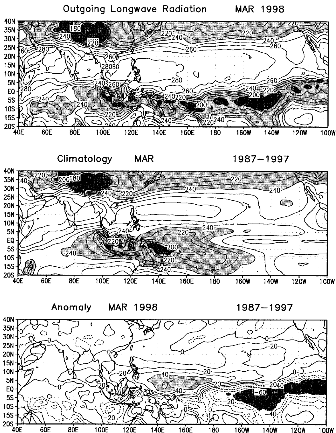
Figure 4b Same as Fig. 4a but for in March 1998.
