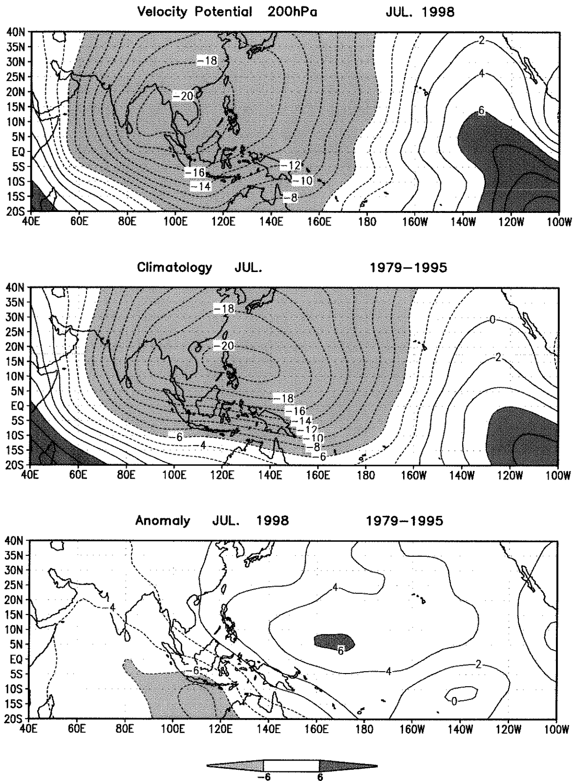
Figure 7d Same as Fig. 7a but for in July 1998.
