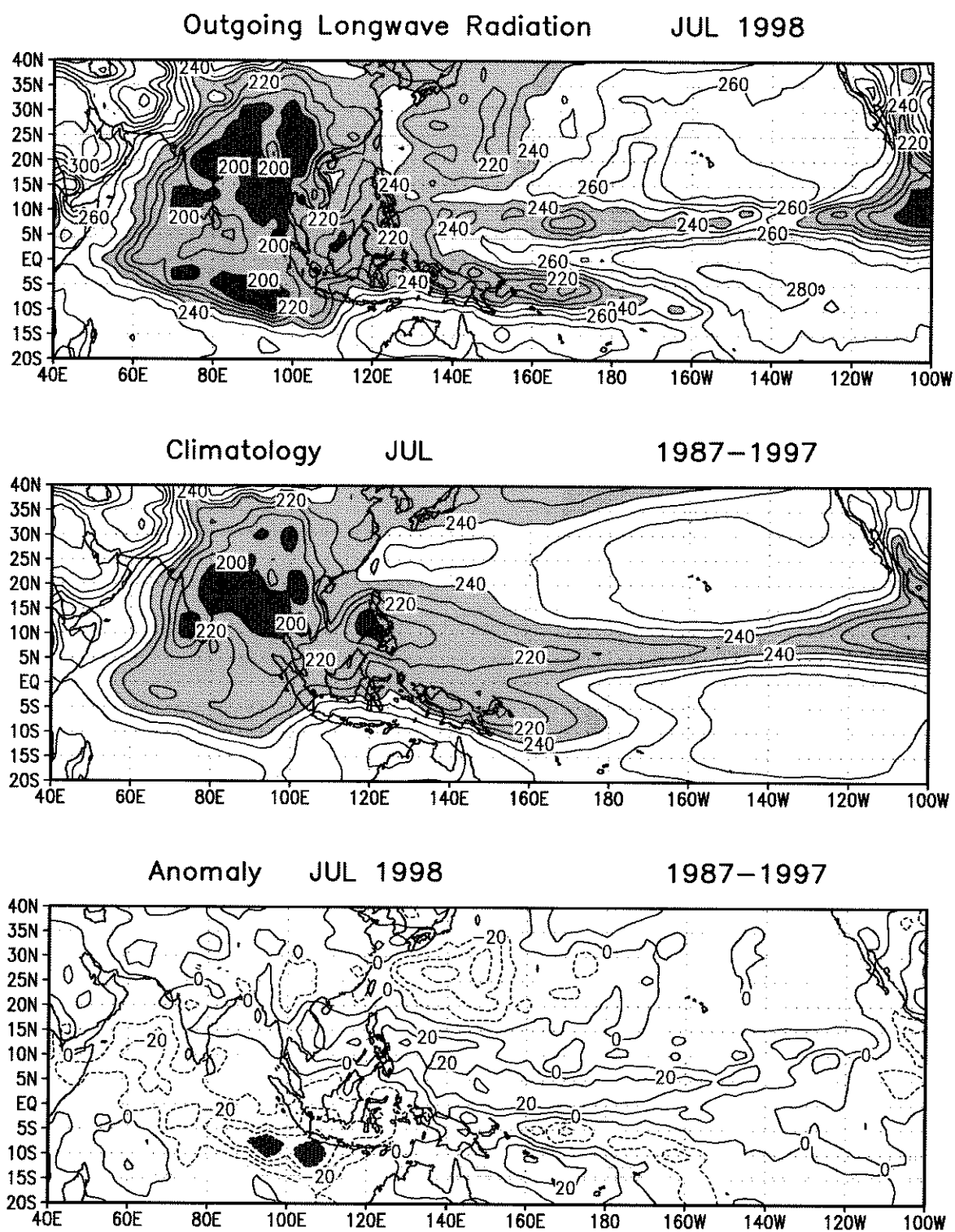
Figure 4d Same as Fig. 4a but for in July 1998.
