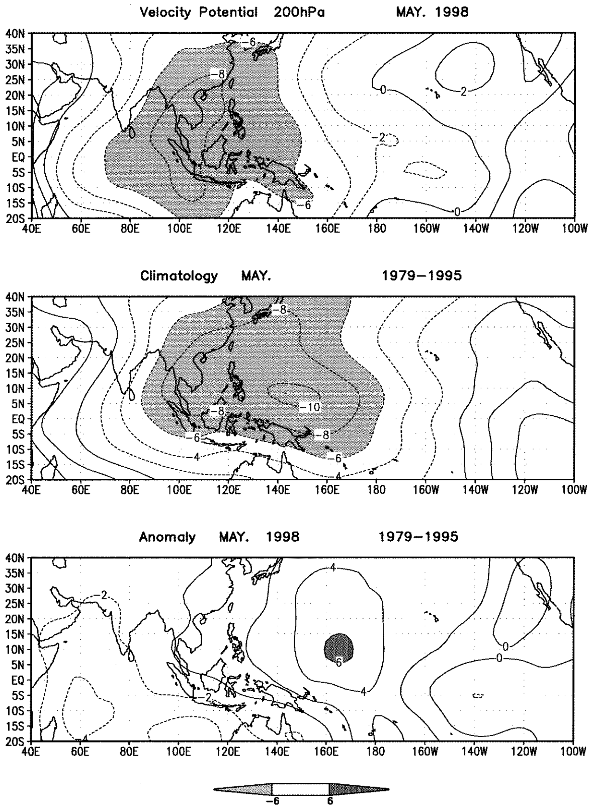
Figure 7c Same as Fig. 7a but for in May 1998.
